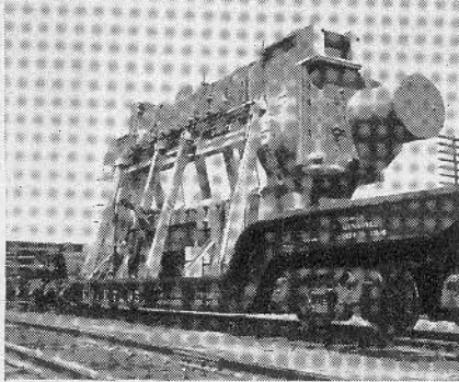
DEPRESSED CENTER FLAT CARS take the big loads, add more clearance inches to Erie's famous high and wide route.
