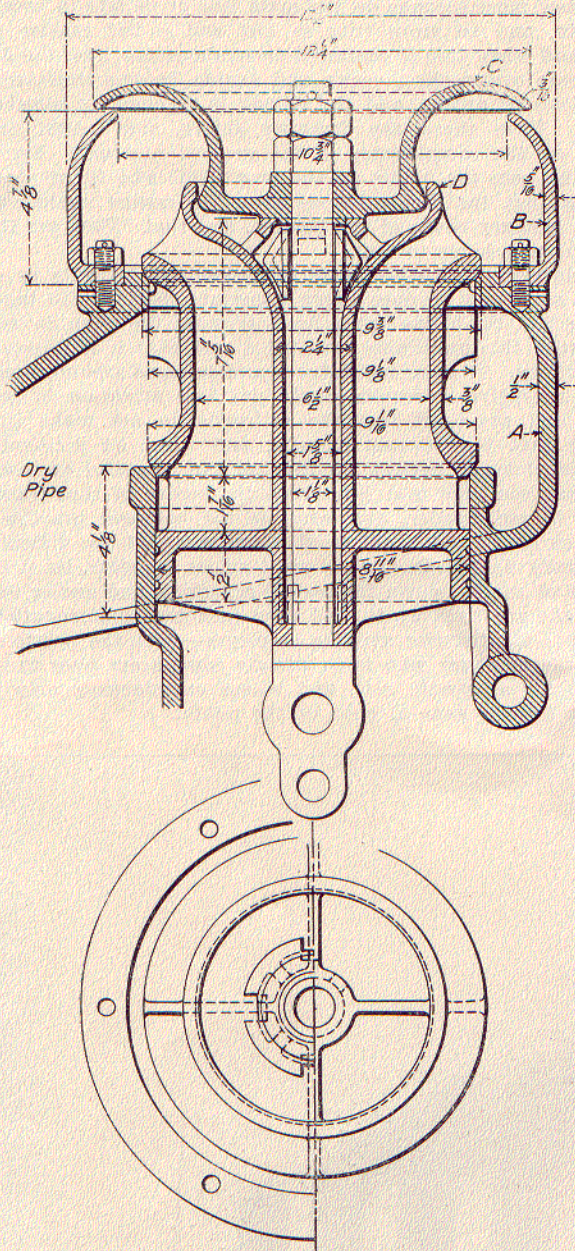
Throttle Valve; Erie Mallet Compound.
