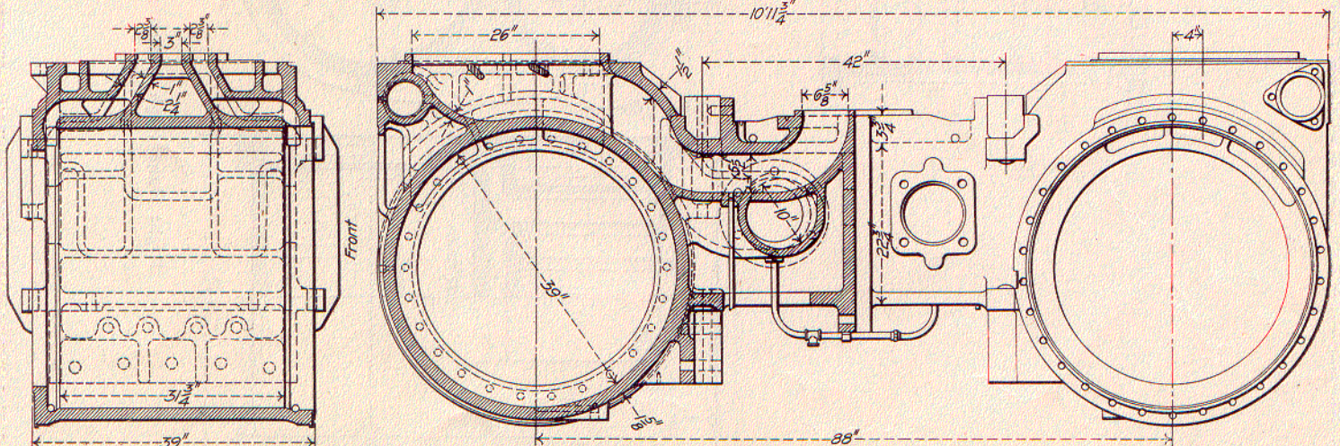
Details of Low Pressure Cylinders; Erie Mallet Compound.
